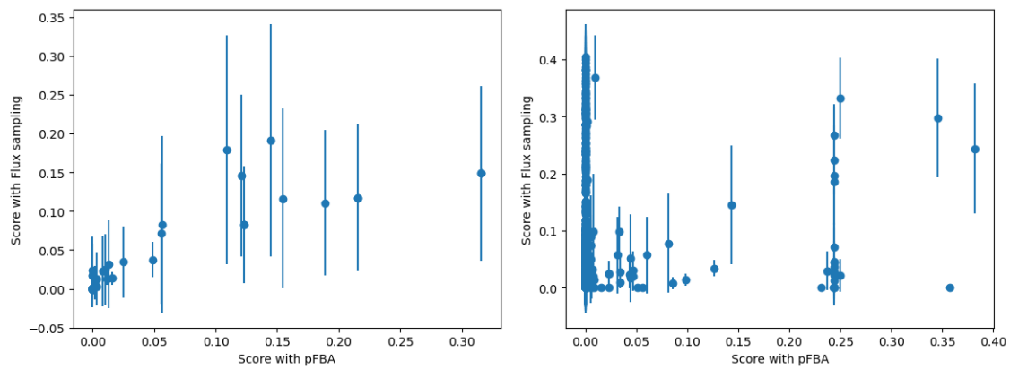
Figure 6. Comparison of the switch scores obtained with pFBA (on the x-axis) versus flux sampling (on the y-axis, with error bars showing standard deviation). A significant correlation was observed for the core metabolic network of E. coli with or without oxygen (left, Spearman correlation: \rho = 0.82 , p = 5.10^{-19} ), but not for the genome scale network of S. cerevisiae with different nitrogen sources (right, for Ala vs Gln, Spearman correlation: \rho = 0.26 , p = 3.10^{-43} ).
