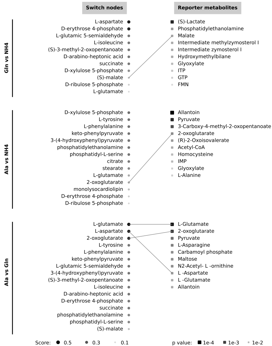
Figure 5. The main switch nodes identified by ISIS for Saccharomyces cerevisiae under nitrogen limitation, in comparison with reporter metabolites computed from transcriptomic data [29].
