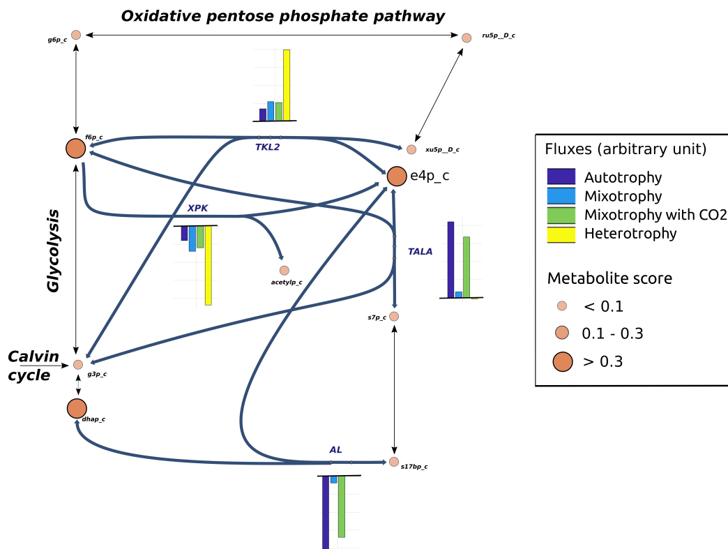
Figure 4. Metabolic fluxes in the non-oxidative pentose phosphate pathway for different trophic modes in the diatom P. tricornutum . Alongside dihydroxyacetone phosphate (dhap) and fructose-6-phosphate (f6p), erythrose 4-phosphate (e4p) appears as a key hub to balance the fluxes between glycolysis, the Calvin cycle and the oxidative pentose phosphate pathway, showing the role of the non-oxidative pentose phosphate pathway in orchestrating the energy balance of the cell.
